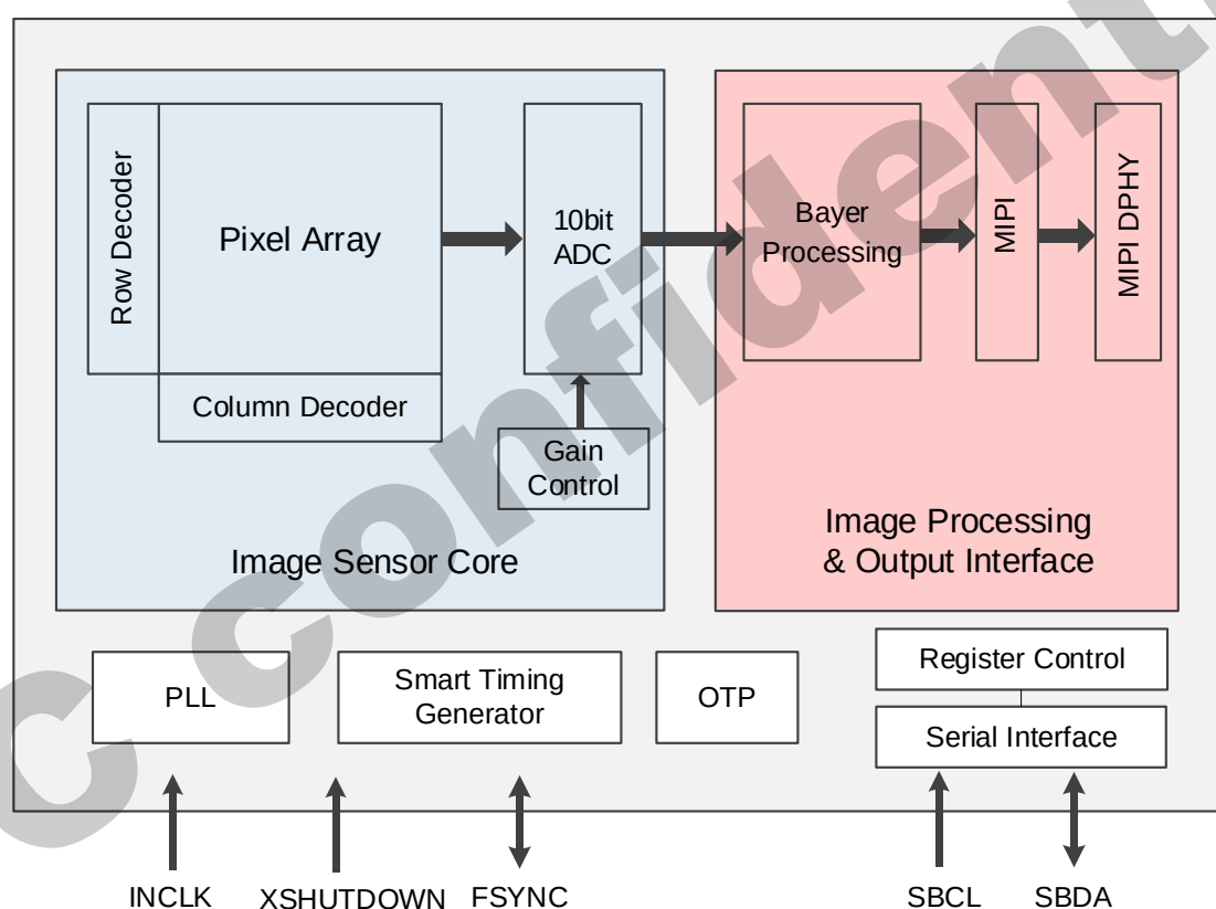
Figure 1: Block Diagram
